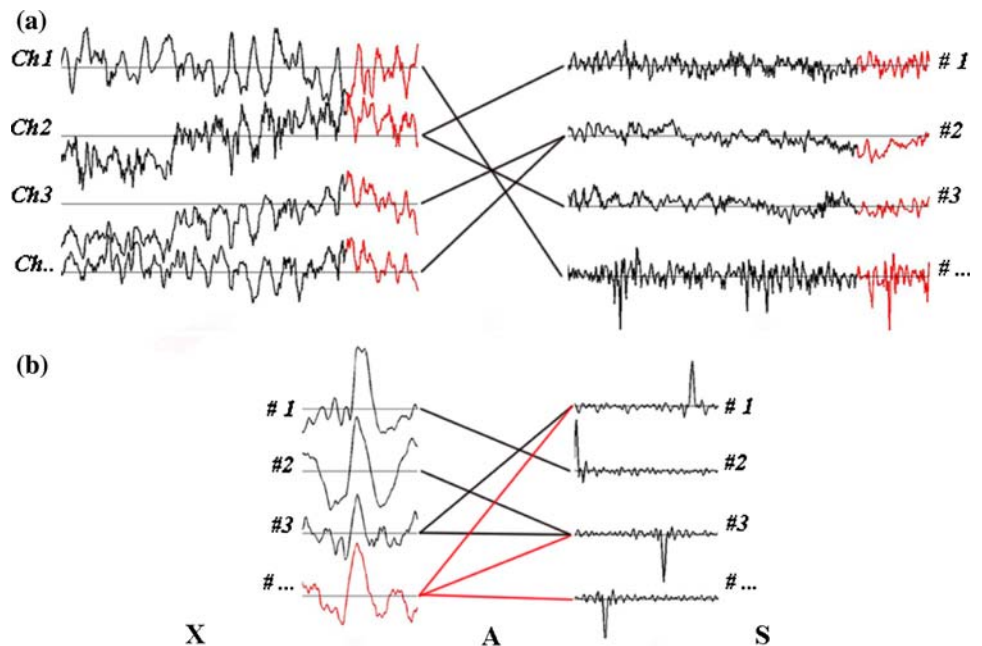
Fig 3 a Temporal ICA: EEG signals ( X ) picked up at some spatial points (Ch1, Ch2, Ch3, ...), can be represented as a linear mixture of independent components ( S ); when new data is measured, the independent components are updated correspondently in time. (b) Our proposed use of ICA: A collection of spikes ( X ) were decomposed into a mixture of independent components ( S ) through the mixing matrix ( A ); when a new spike was added to the dataset of spikes ( S ) was kept fixed and the mixing matrix ( A ) was updated. The four independent components represented here were a subset of the whole set of 105 independent components obtained from one of the cross validation split of our dataset
