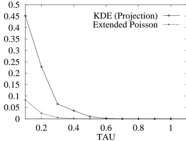
Figure 11: The expected error ( E ) in the decoded distribution, averaged over 50 samples from the firing rate distributions, is plotted against different values of \tau , the width of the bimodal gaussian implicit distribution. The results for only one of the KDE methods are shown because both KDE methods involve the same decoding operation.
