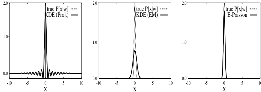
Figure 4: The KDE method has difficulty capturing the high-frequency information in the implicit gaussian distribution, when its standard deviation, \tau = 0.2 , is smaller than the kernel widths ( \sigma = 0.3 ).
