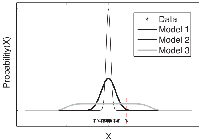
Figure 2: Model complexity and evidence. See text for details.
