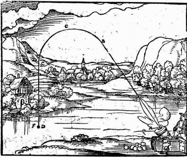
Figure 1: The renaissance view of projectile motion was conceptually complex. It divided the trajectory into several parts (two straight and one curved!) and included an account of the interaction of the projectile with the atmosphere. Though intuitively satisfactory, it was computationally intractable and ultimately misleading. Image downloaded from http://tinyurl.com/34p9up6 .
